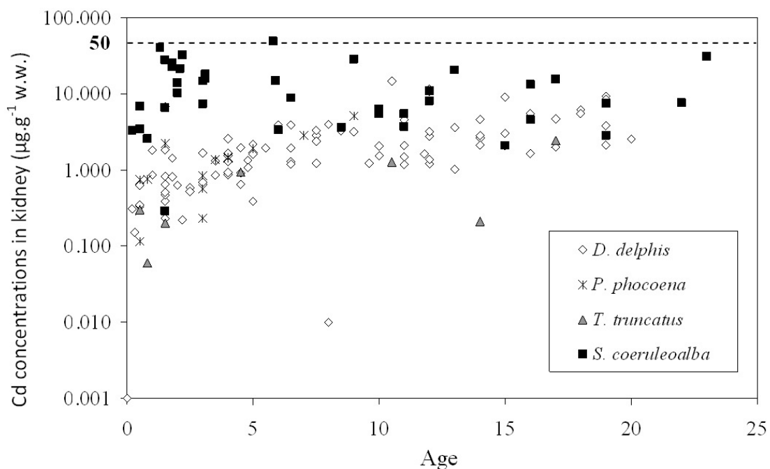
Figure 2: Bioaccumulation of cadmium in kidney ( \mu\text{g/g wt} ) with age (years) in small cetaceans from the Bay of Biscay. The Threshold Limit Value of 50 \mu\text{g.g}^{-1} \text{w.w.} is indicated (see text). (modified from Lahaye et al. , 2004; Lahaye, 2006)
