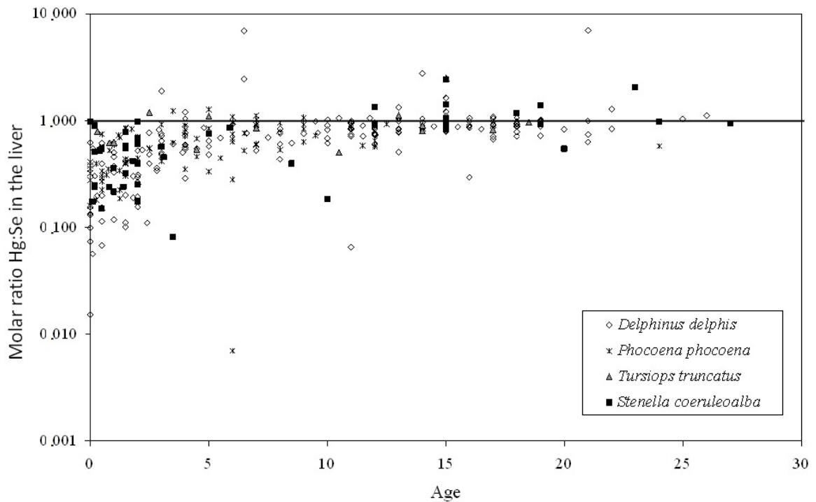
Figure 8. Relationship between molar ratio Hg:Se in liver tissue and age in small cetaceans from the European Waters. The line indicates 1:1 molar ratio. (from Lahaye, 2006)
