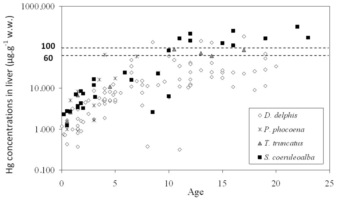
Figure 7. Bioaccumulation of mercury in liver ( \mu\text{g/g wt} ) with age (years) in small cetaceans from the Bay of Biscay. The Threshold Limit Value of 60 \mu\text{g.g}^{-1} w.w and 100 \mu\text{g.g}^{-1} are indicated (see text). (modified from Lahaye et al. , 2004; Lahaye 2006).
